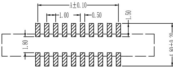
PCB Layout
